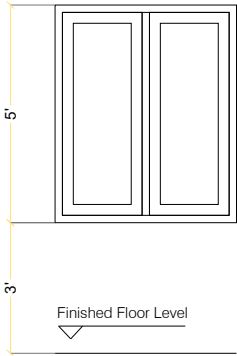
ELEVATION VIEW
