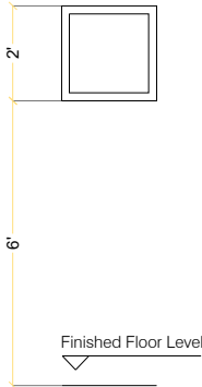
ELEVATION VIEW
