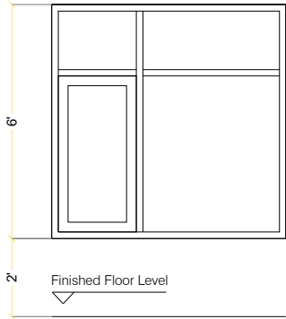
ELEVATION VIEW
